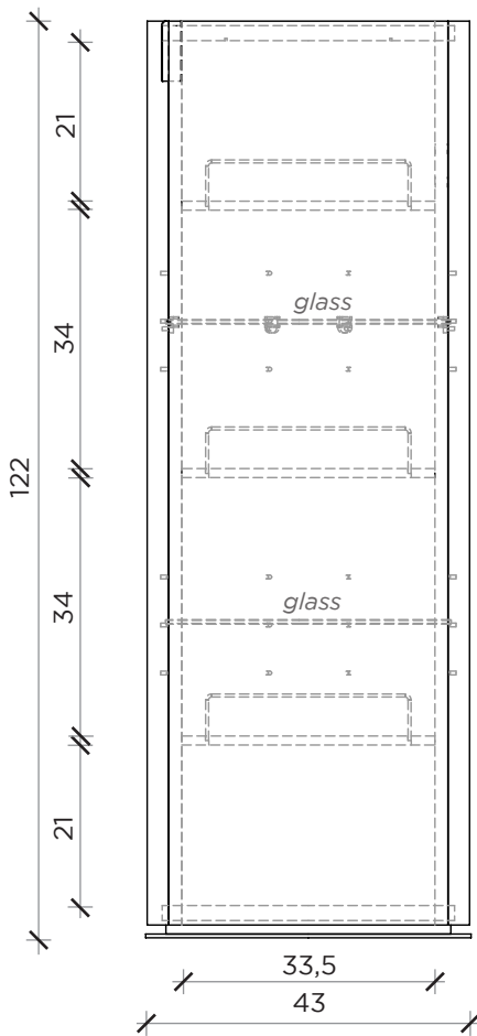
FRONTE | FRONT
