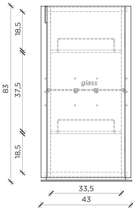
FRONTE | FRONT
