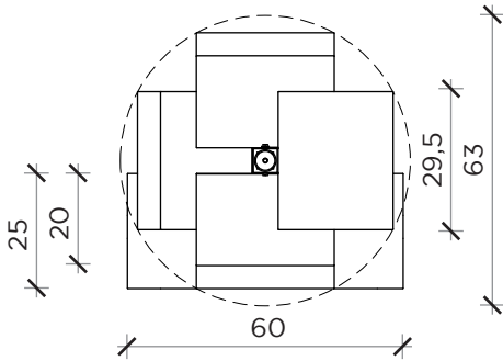
FRONTE | FRONT
