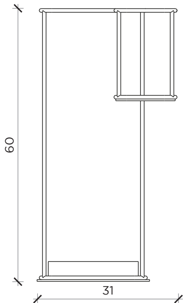
FRONTE | FRONT
